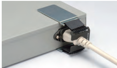
●ハブへ装着 Attached to Hub
